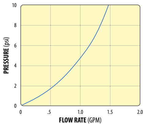
250 BARB Flow Rate vs. Pressure
