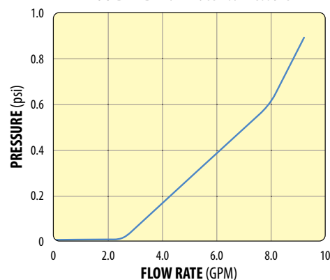
700 BARB Flow Rate vs. Pressure
