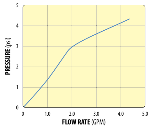
400 BARB Flow Rate vs. Pressure
